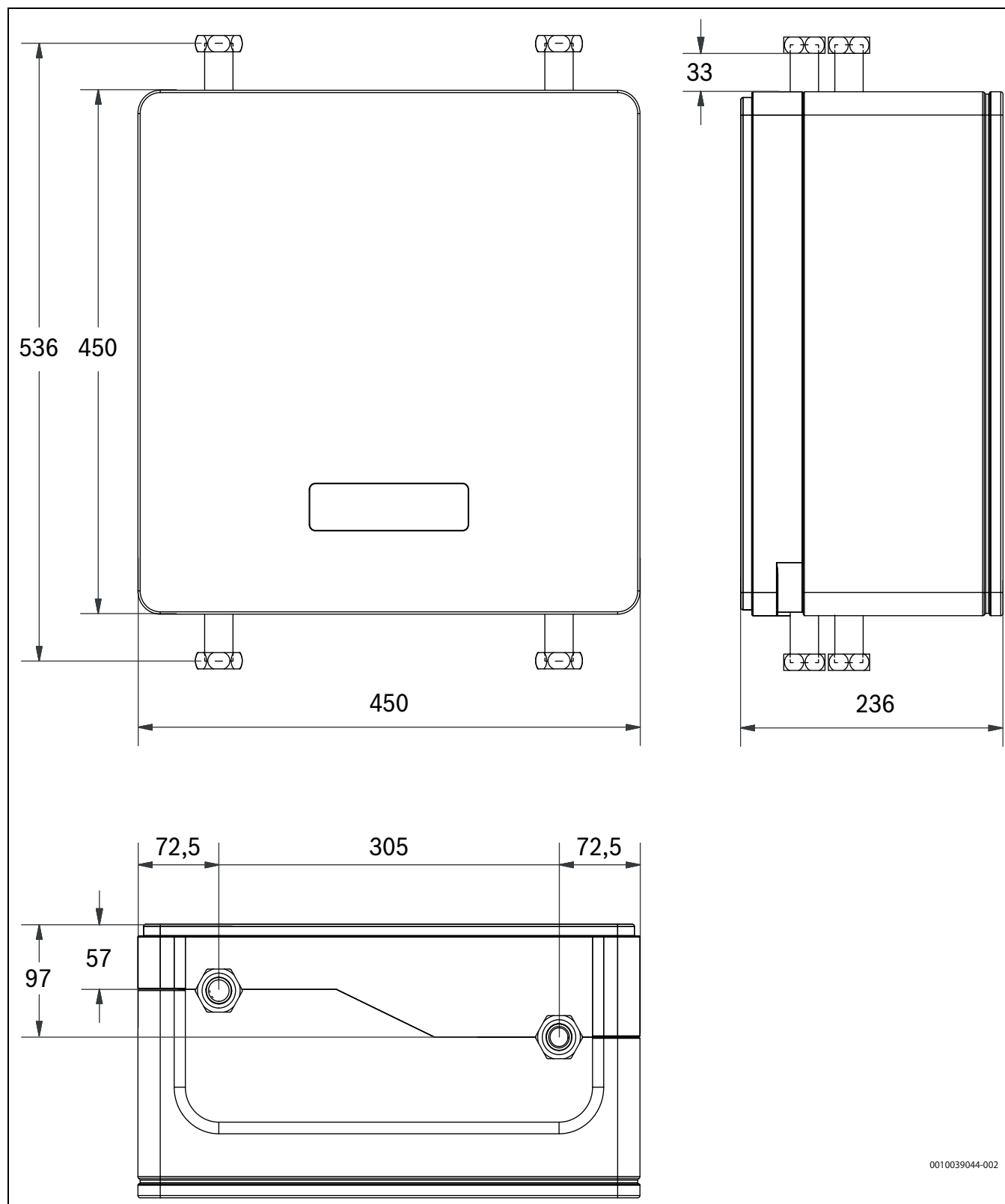
Fig. 3 Dimensions, raccordements
