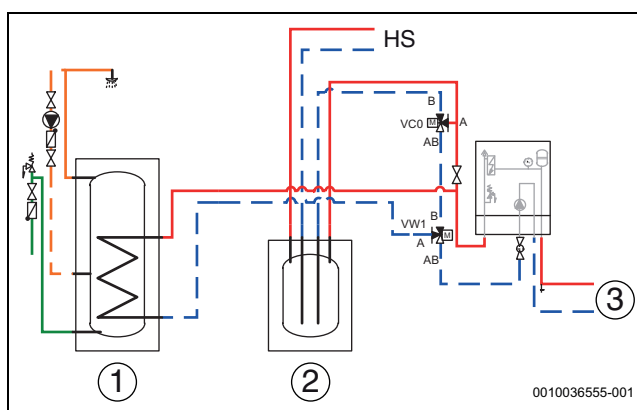
Fig. 29 Tampon, vanne bypass VC0
